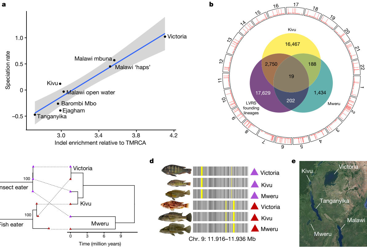
Fig. 2 | Large indels are associated with speciation and adaptation across cichlid radiations. a , Positive association between speciation rate (phylogenetic mean of the \log_{10} -transformed DR statistic; see Supplementary Information section 2.2 for additional speciation rate metrics) and the number of linkage-disequilibrium-filtered indels with a length of at least 5 bp relative to the TMRCA. The blue line indicates the regression line from a linear regression; grey shading shows the 95% confidence intervals of the mean. Indels are measured using genome pairs from Lake Tanganyika lamprologines, Barombi Mbo oreochromines, Ejagham Coptodon , Kivu haplochromines, Malawi open-water Rhamphochromis / Diplotaxodon / Pallidochromis , the ecologically diverse Malawi haplochromine clade known as 'haps', Malawi mbuna, and the Lake Victoria haplochromine species flock. b , Venn diagram of indels ( n = 38,689 ) that segregate between species in the Lake Victoria radiation that also segregate either within Lake Kivu, Lake Victoria Region Superflock (LVRS) founding lineages and/or Lake Mweru. The outer ring shows the genomic positions of ancient large indels that were significantly associated with diet, habitat or nuptial coloration ( n = 214 ). c , Phylogeny of the region on
